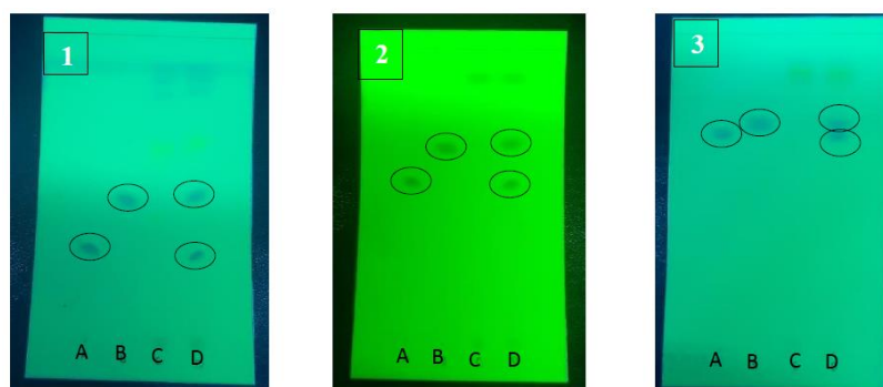
Figure 1. Elution from three different mobile phase
